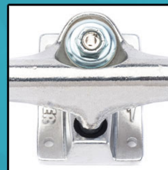
AIRCRAFT GRADE HOLLOW KINGPINS
